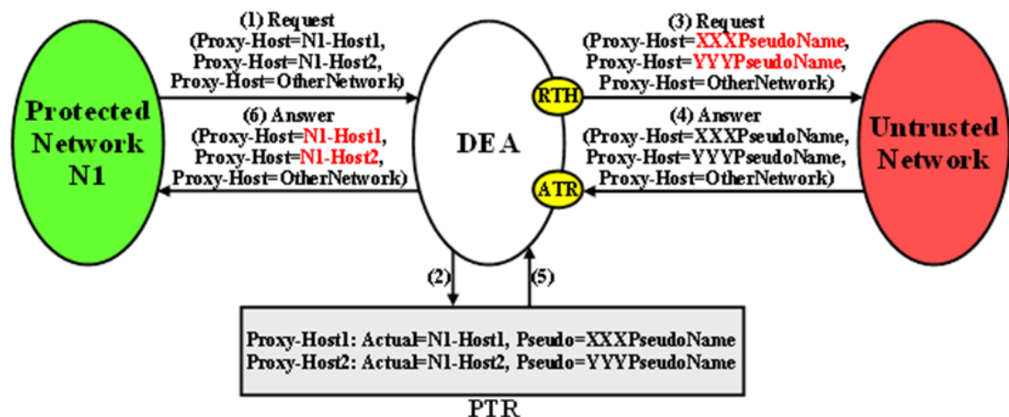
Figure 9-10 Proxy-Host Hiding
